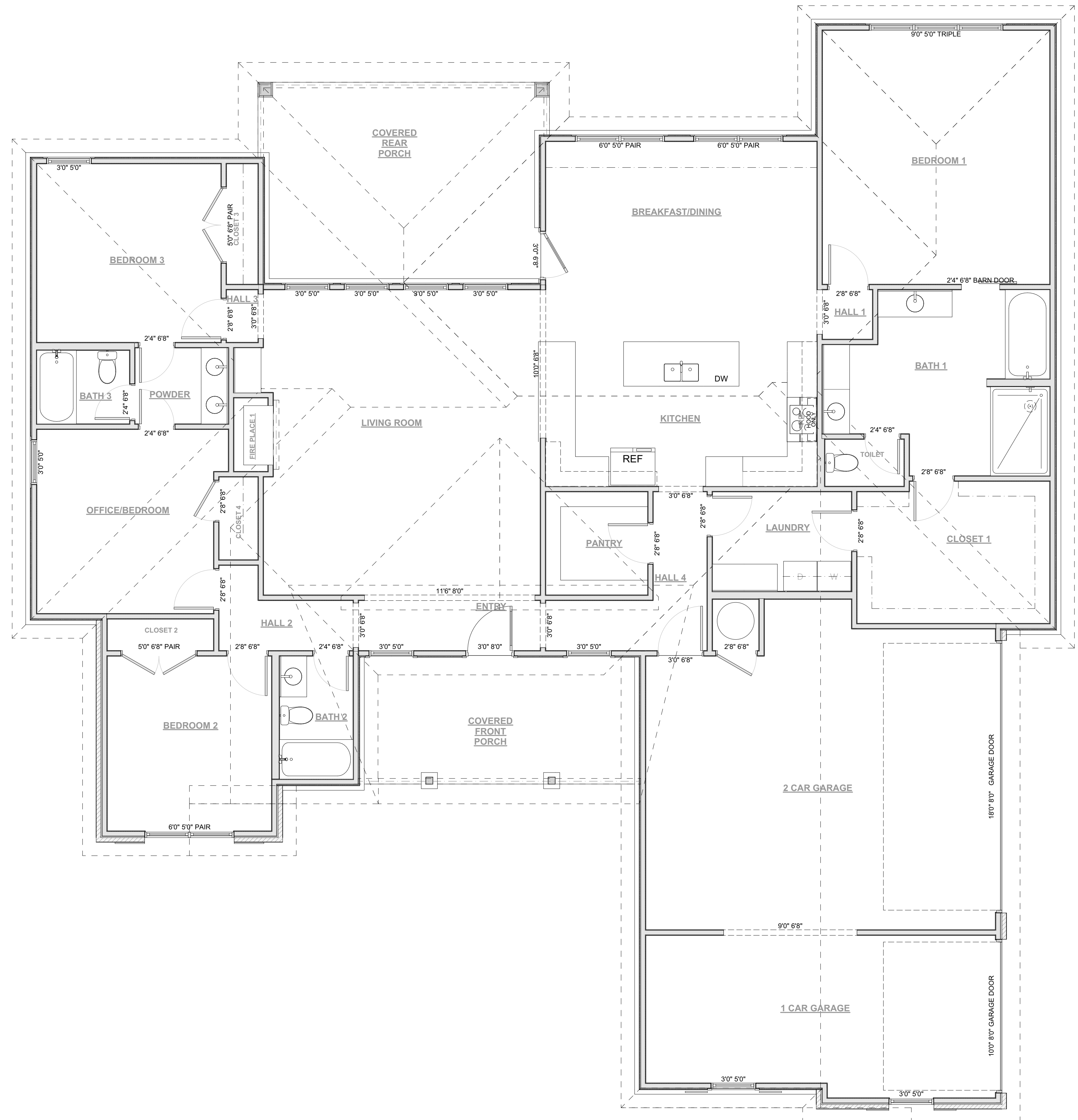
1 FLOOR PLAN
