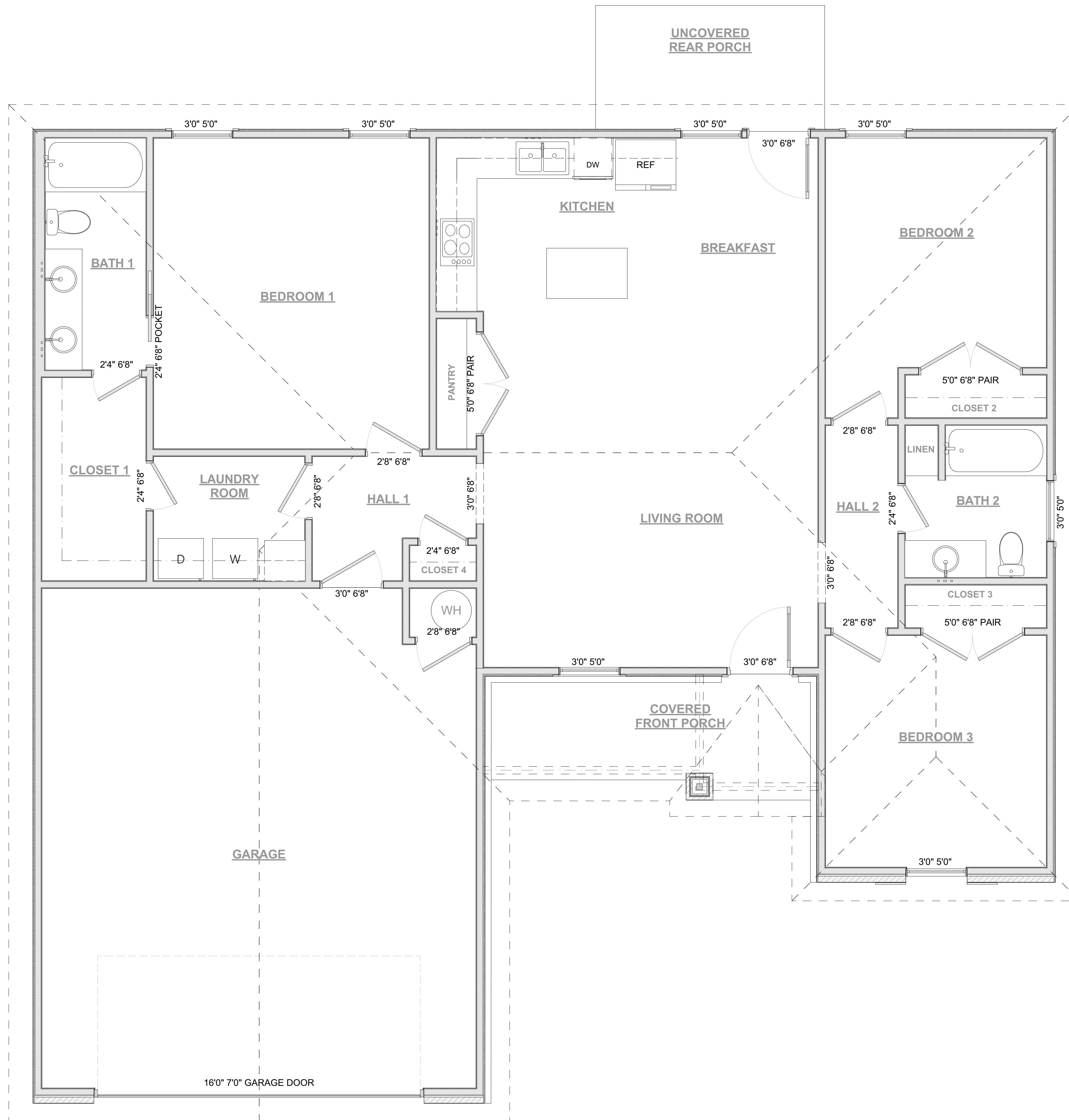
1 FLOOR PLAN 1,401 sq ft ## SCALE: 3/8" = 1'-0"
