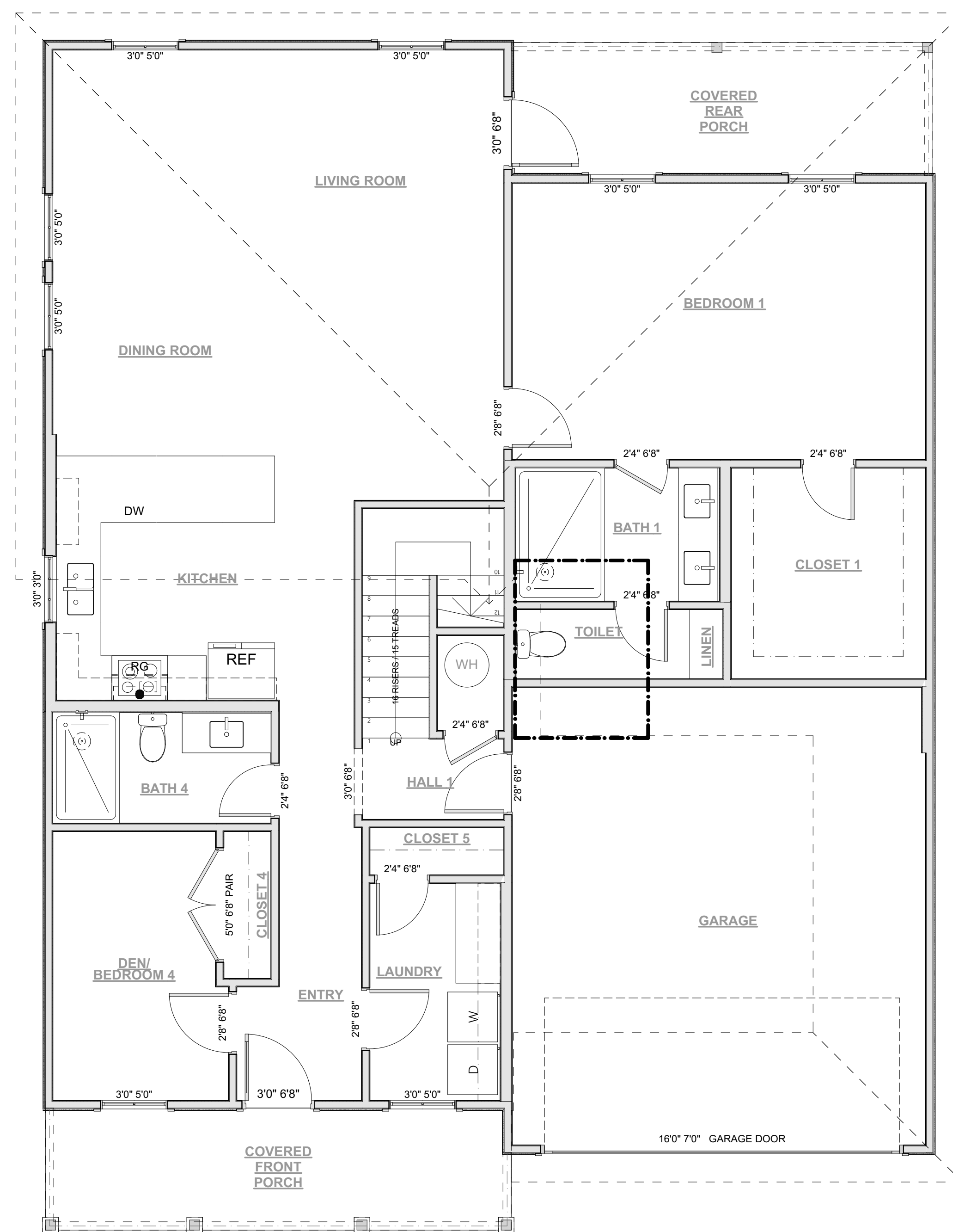
1 GROUND FLOOR PLAN 00 1,461 sq ft
