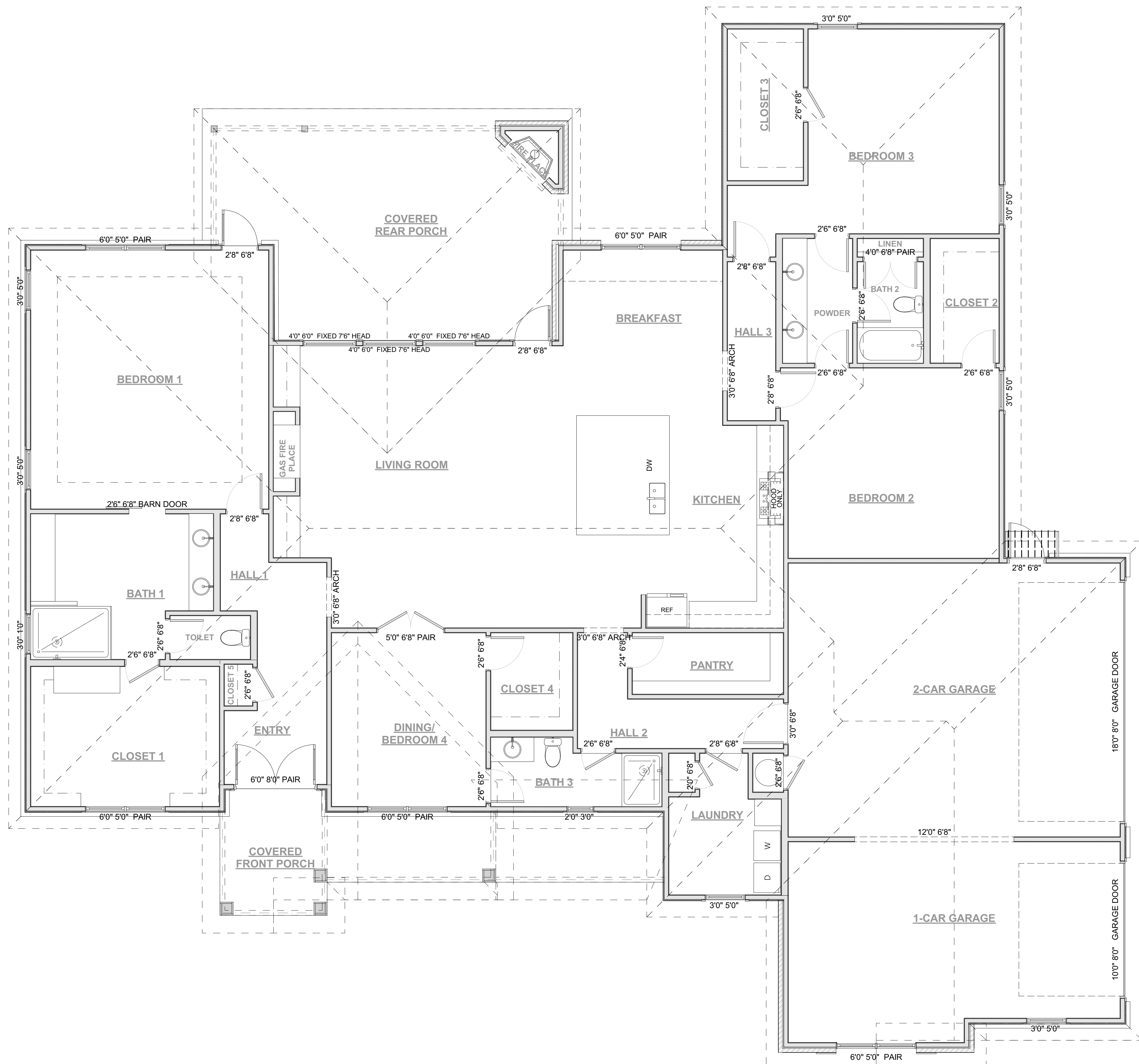
1 FLOOR PLAN 00
