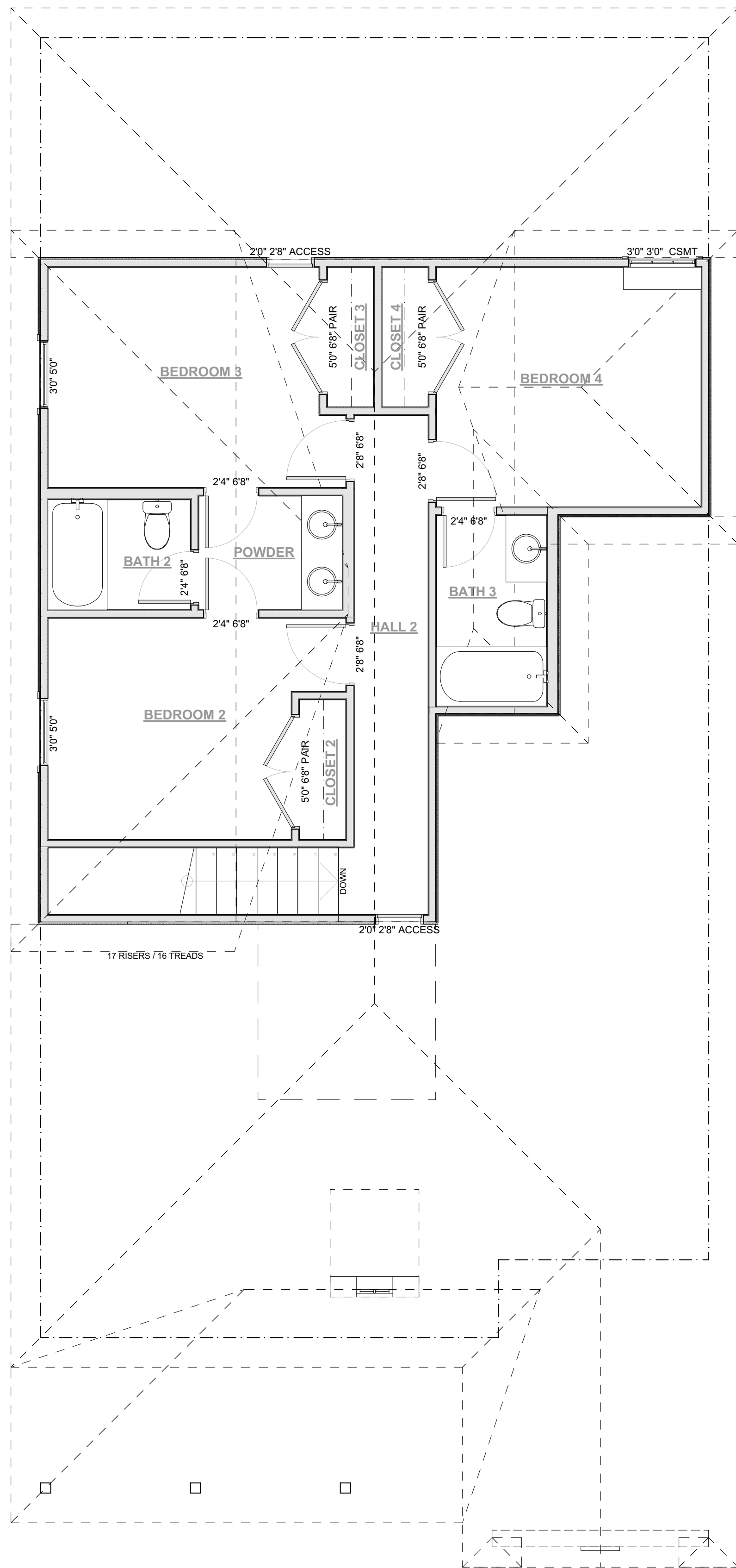
2 UPPER FLOOR PLAN DT00 687 sq ft
