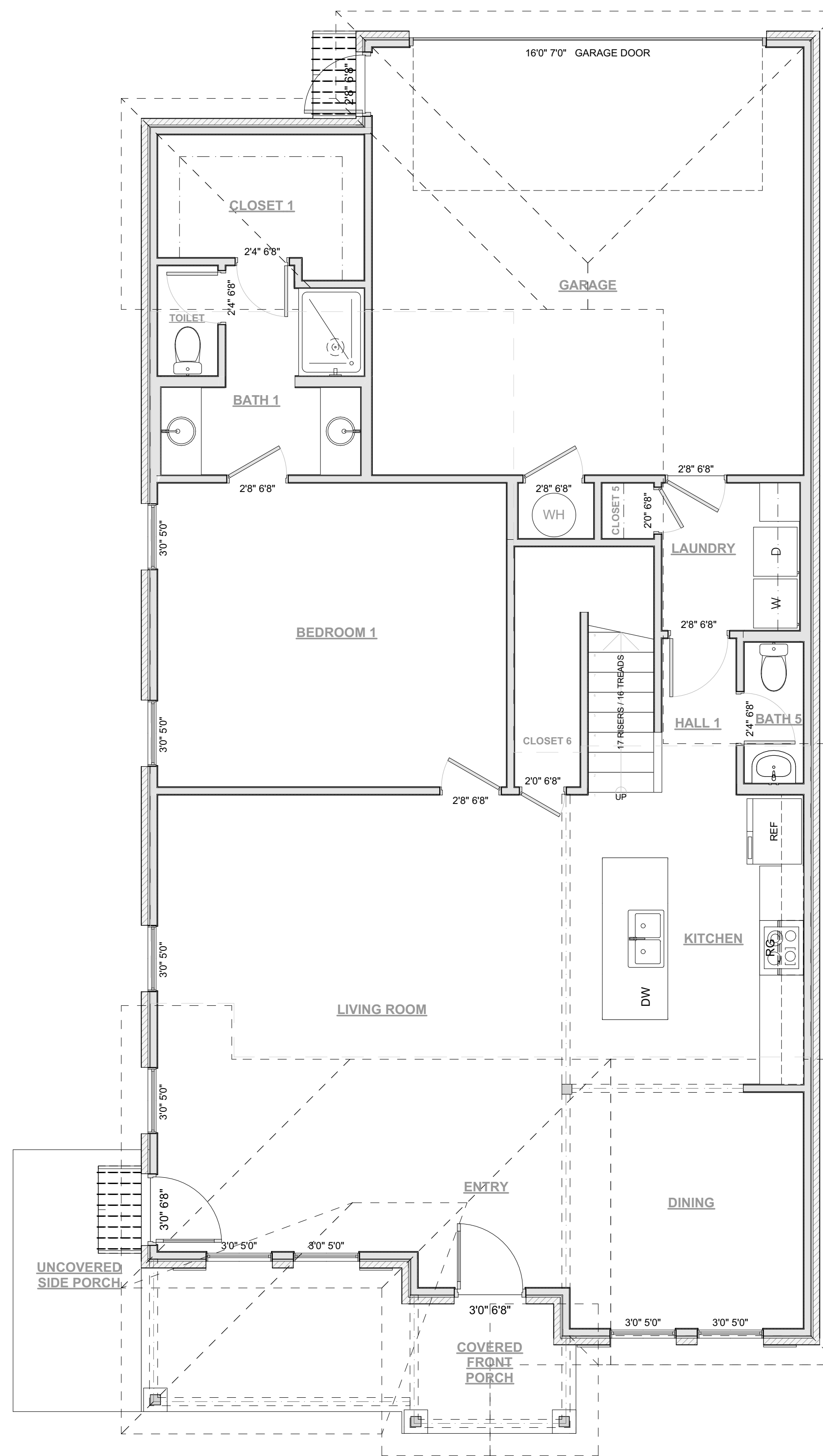
1 GROUND FLOOR PLAN DT00 1,346 sq ft
