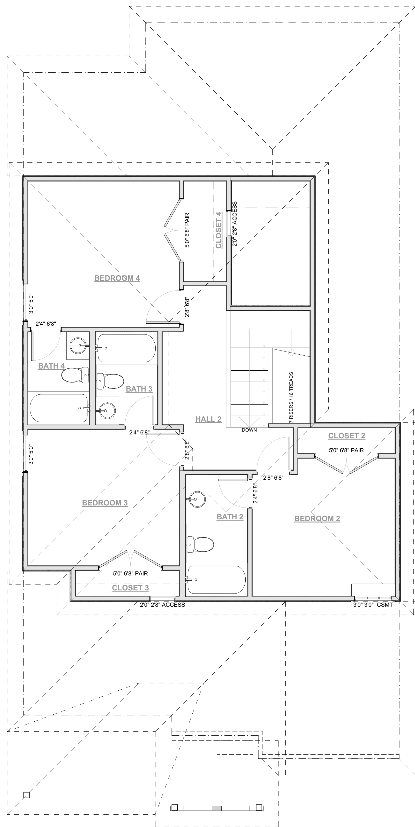
2 UPPER FLOOR PLAN DT00 764 sq ft
