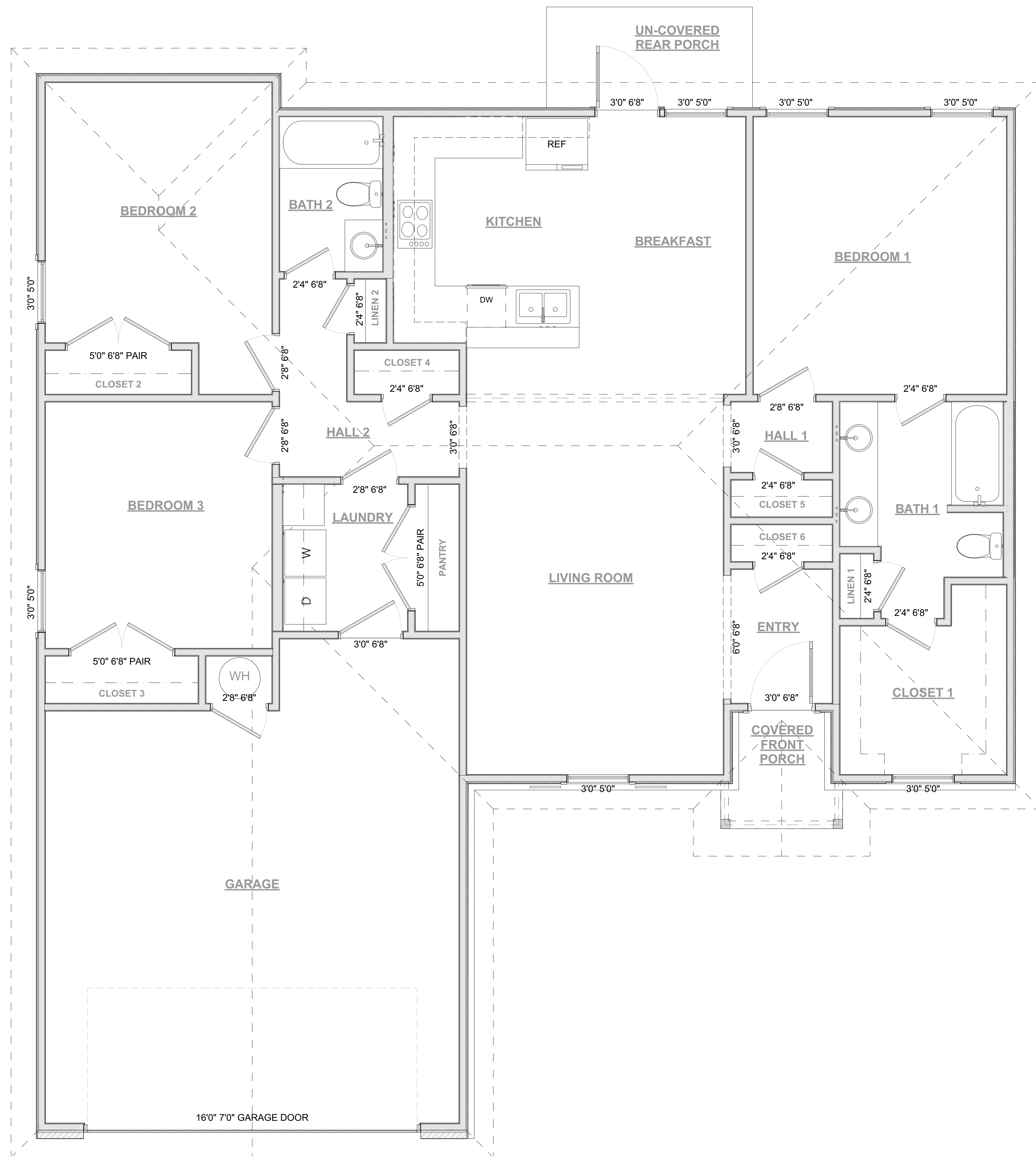
1 FLOOR PLAN 1,450 sq ft ## SCALE: 3/8" = 1'-0"
